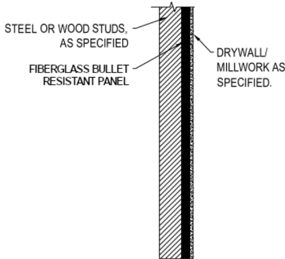
SECTION VIEW
