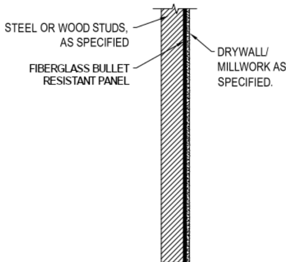
SECTION VIEW
