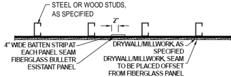
PLAN VIEW
